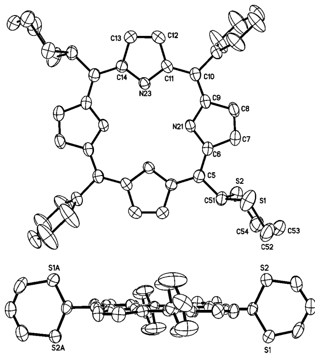
Figure 1. Top and side view of the molecular structure of 16b in the crystal. Thermal ellipsoids are drawn for 50% occupancy; hydrogen atoms are omitted for clarity.
