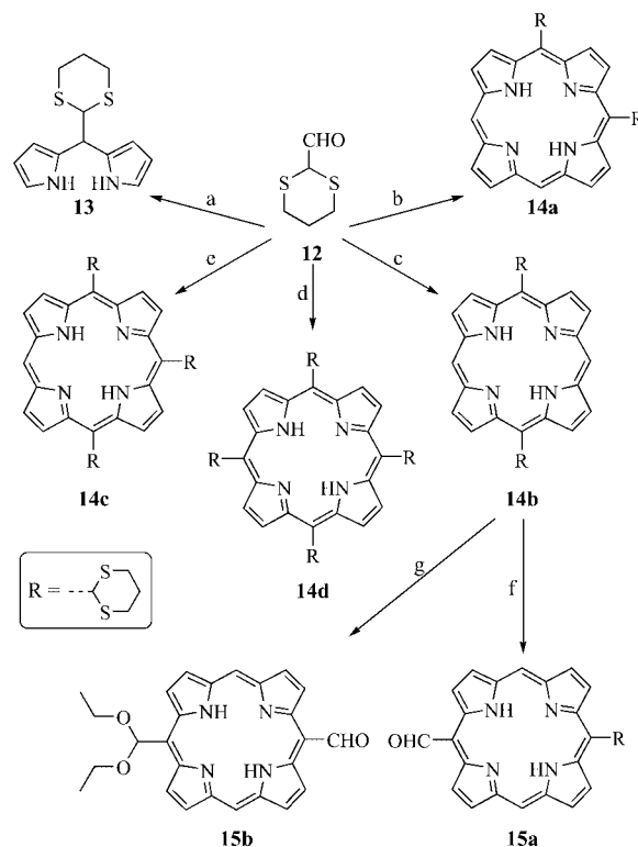
Scheme 3. Condensation reactions involving dithian-2-carbaldehyde. Conditions: (a) pyrrole, \text{BF}_3 \cdot \text{OEt}_2 , room temp., 40 min, then NaOH, 96%. (b) \text{CH}_2\text{Cl}_2 , tripyrrane, pyrrole, 45 min, room temp.; then TFA, room temp., 16 h; then DDQ; then \text{NEt}_3 , 3%. (c) \text{CH}_2\text{Cl}_2 , dipyrromethane, TFA, 14 h, room temp.; then DDQ, 10 min, reflux, 16%. (d) \text{CH}_2\text{Cl}_2 , pyrrole, \text{BF}_3 \cdot \text{OEt}_2 , 1 h, room temp.; then \text{NEt}_3 , DDQ, 4 min, 15%. (e) \text{CH}_2\text{Cl}_2 , pyrrole, \text{BF}_3 \cdot \text{OEt}_2 , 1 h, room temp.; then excess DDQ, 1 h, 46%. (f) \text{CHCl}_3 , 8 equiv. bis(trifluoroacetoxy)iodobenzene (BTIB), 45 °C, 30 min, 62%. (g) \text{CHCl}_3 , 4 equiv. BTIB, room temp., 30 min, 30%.
