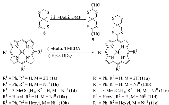
Scheme 2. Synthesis of spirobisdithiane derivatives.
