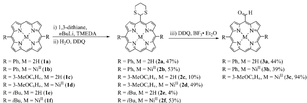
Scheme 1. Formylation of porphyrins by the 1,3-dithian-2-yl synthon.
