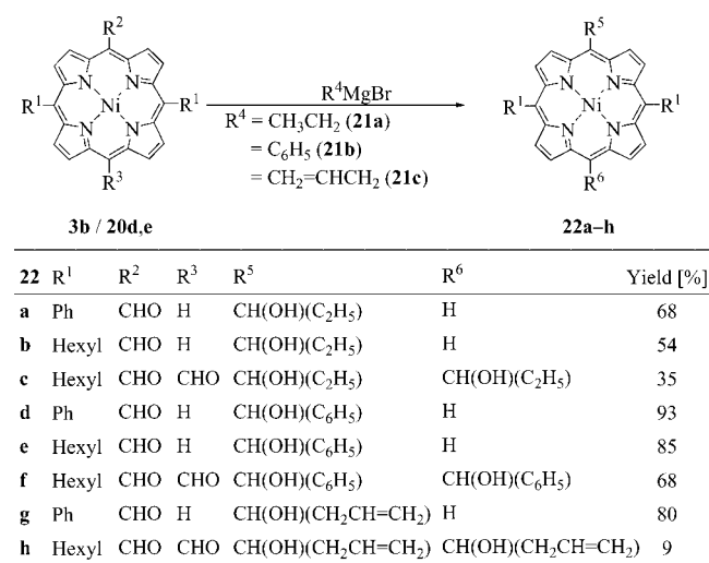
Scheme 6. Grignard reactions.
