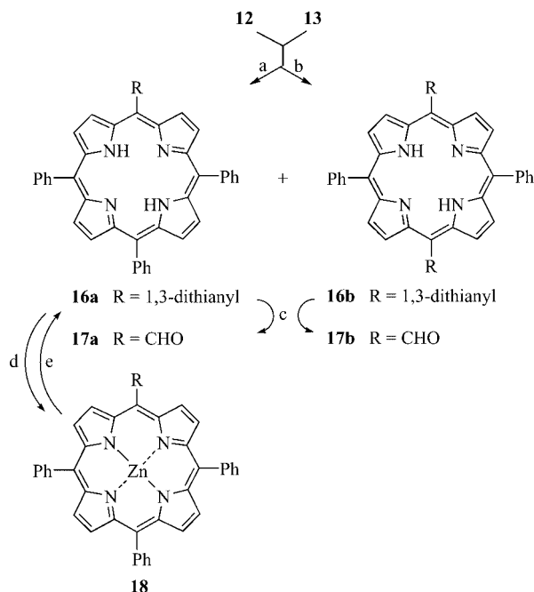
Scheme 4. meso -Substituted dithian-2-ylporphyrins. Conditions: (a) \text{CH}_2\text{Cl}_2 , 5-phenyldipyrromethane, cat. TFA, 16 h, room temp.; then DDQ, 45 min, 16a 3%, 16b 2%. (b) \text{CH}_2\text{Cl}_2 , benzaldehyde, cat. TFA, 16 h, room temp., then DDQ, 45 min, 16a 2%, 16b 4%. (c) \text{CH}_2\text{Cl}_2 , DDQ, \text{BF}_3 \cdot \text{OEt}_2 , room temp., 10 min, 97%. (d) \text{CH}_2\text{Cl}_2 , \text{ZnOAc} , \text{CH}_3\text{OH} , room temp., 30 min, 53%. (e) \text{H}_2\text{SO}_4 .
