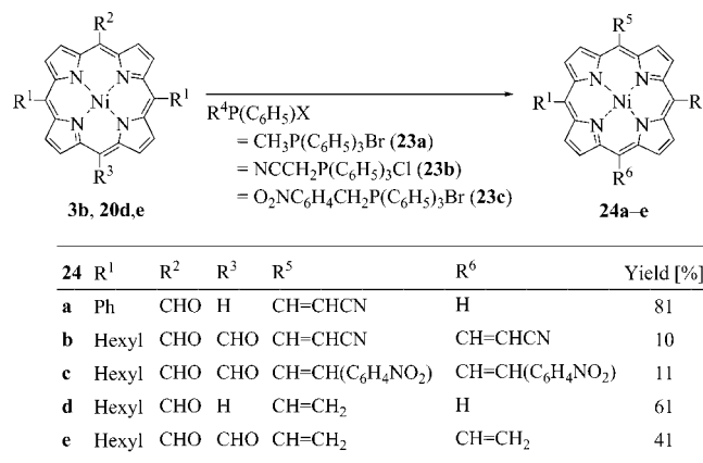
Scheme 7. Wittig reactions.
